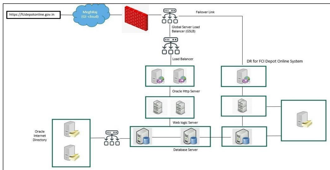
Figure 5: Current DOS DC-DR Architecture
